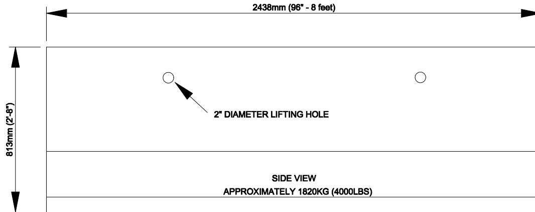
12" x 8' JERSEY BARRIER
