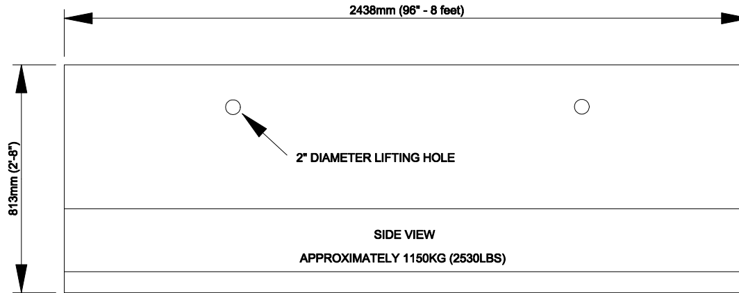
6" x 8' JERSEY BARRIER
